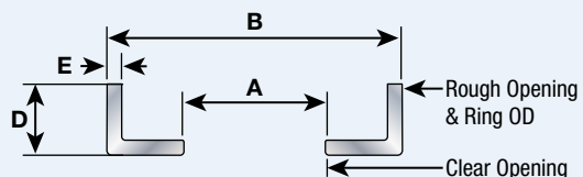
S-C Steel Deck Ring with Compression Seal
